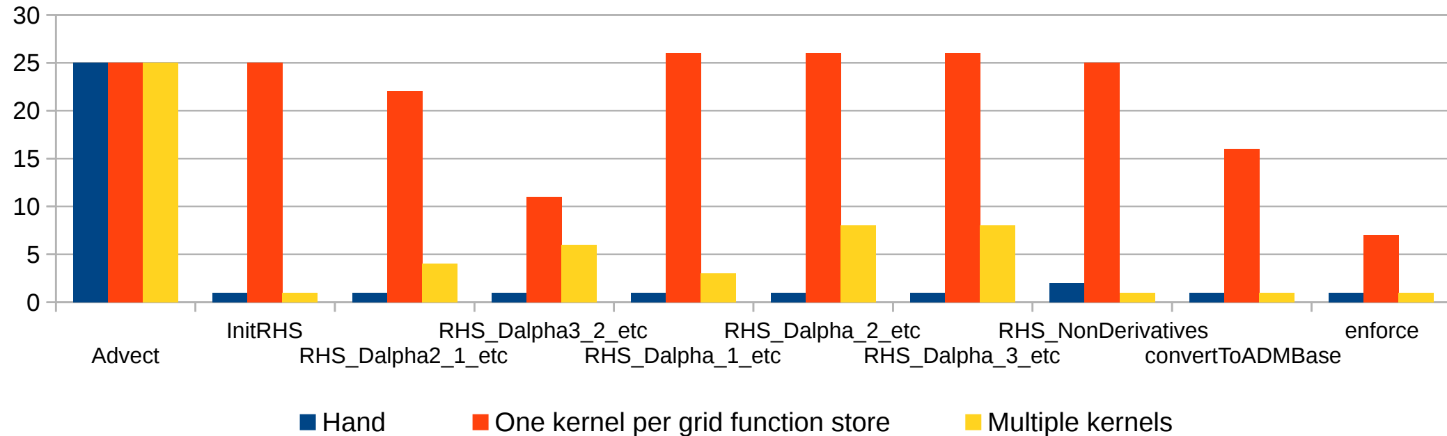
Number of generated CUDA kernels per computation
