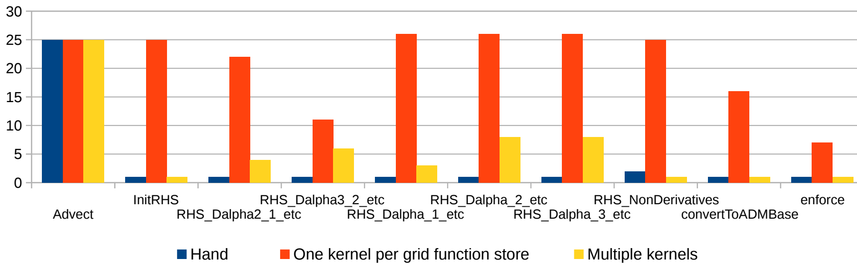
Number of generated CUDA kernels per computation
