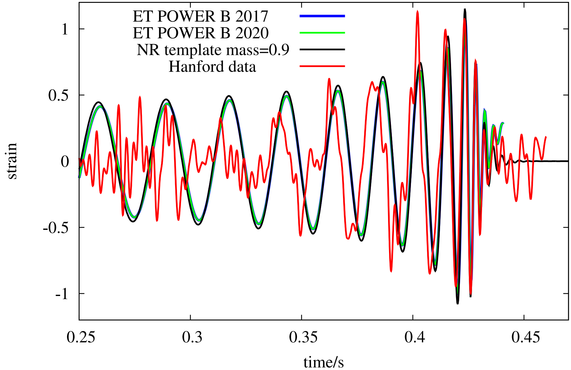
Strain GW150915: ET-2020-05, NR template and Hanford data
